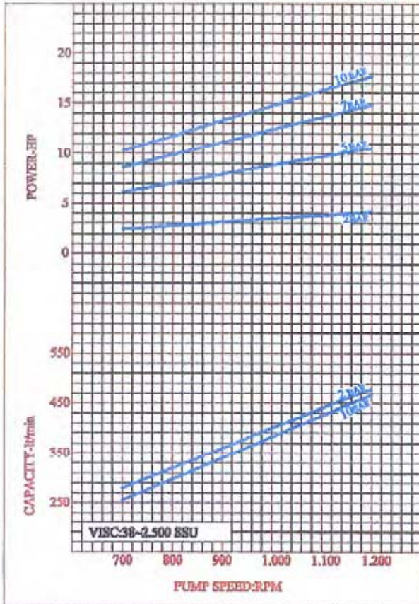
CURVE NO: XLCB-01
